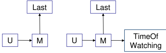
Figure 3: Left: As additional information, the last movie, which the user has watched, is added. Right: The month when the user watches the movie is added.
