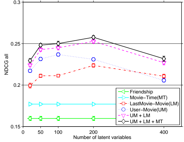
Figure 4: Experiments with social networks data without model regularization. NDCG score as a function of s , the rank in the matrix completion.
