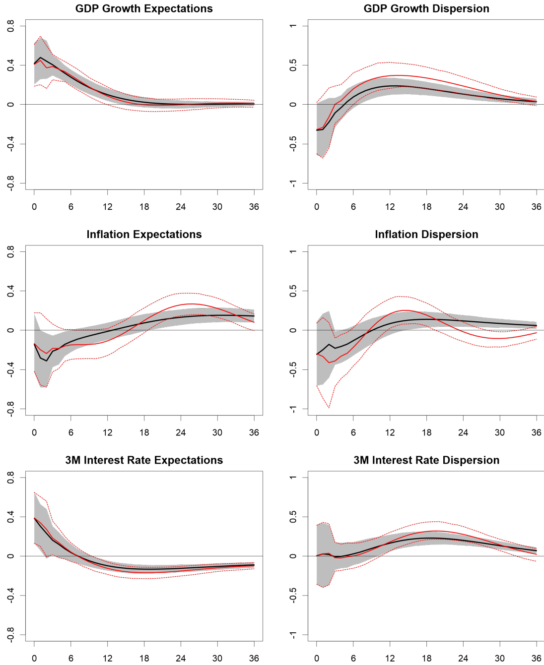
Figure 3: IRFs for Cyclical Size Factor ( \widetilde{SMB} )
