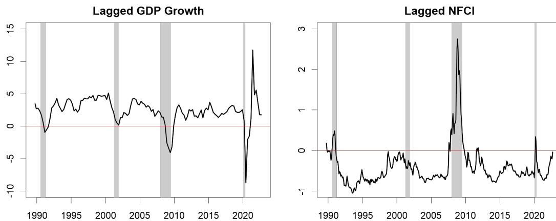
Figure A4: State Drivers for Logit-Mixture Weights
