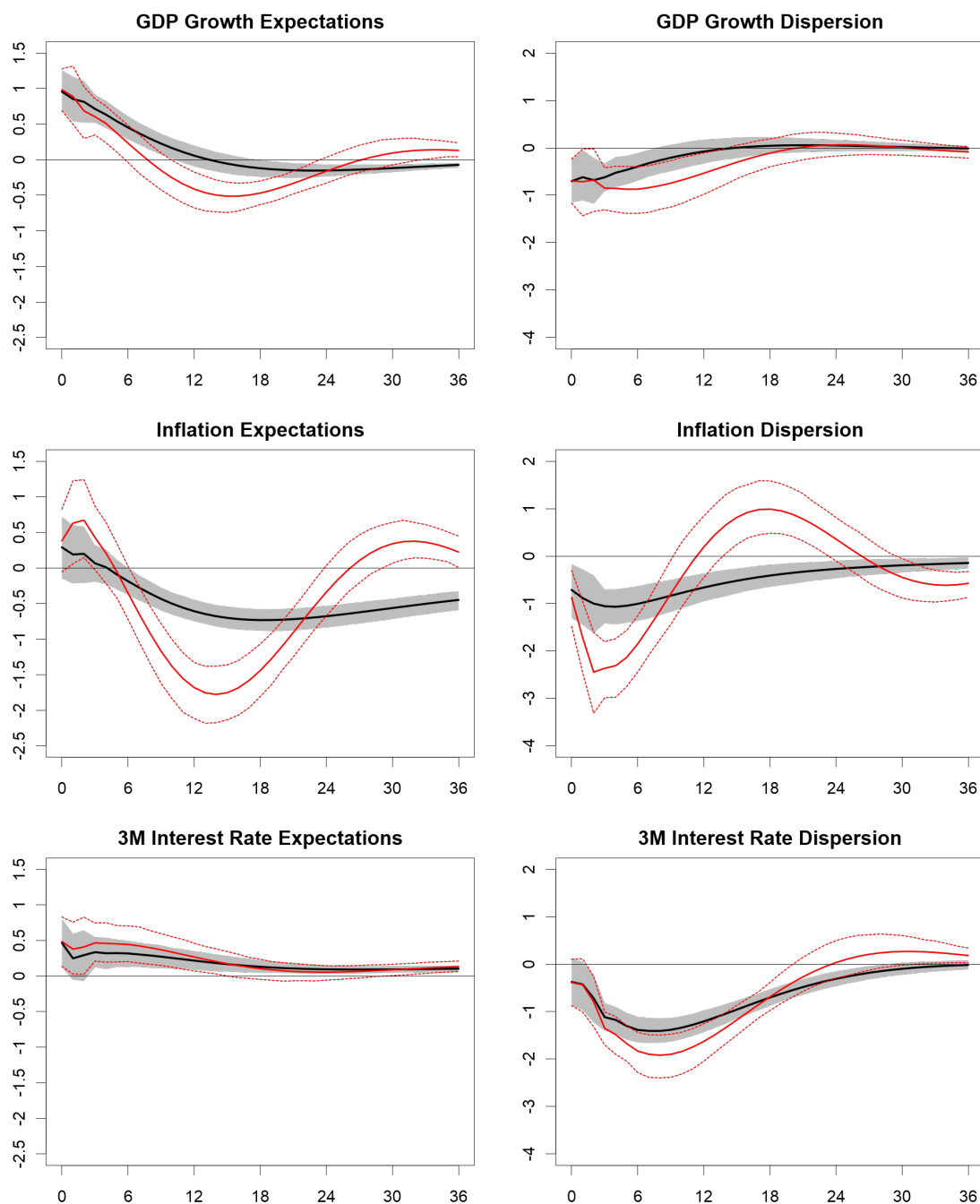
Figure 2: IRFs for Cyclical Market Factor ( \widetilde{MKT} )
