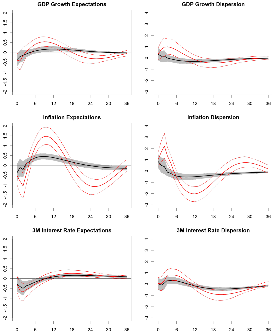
Figure 5: IRFs for Cyclical Momentum Factor ( \widetilde{MOM} )
