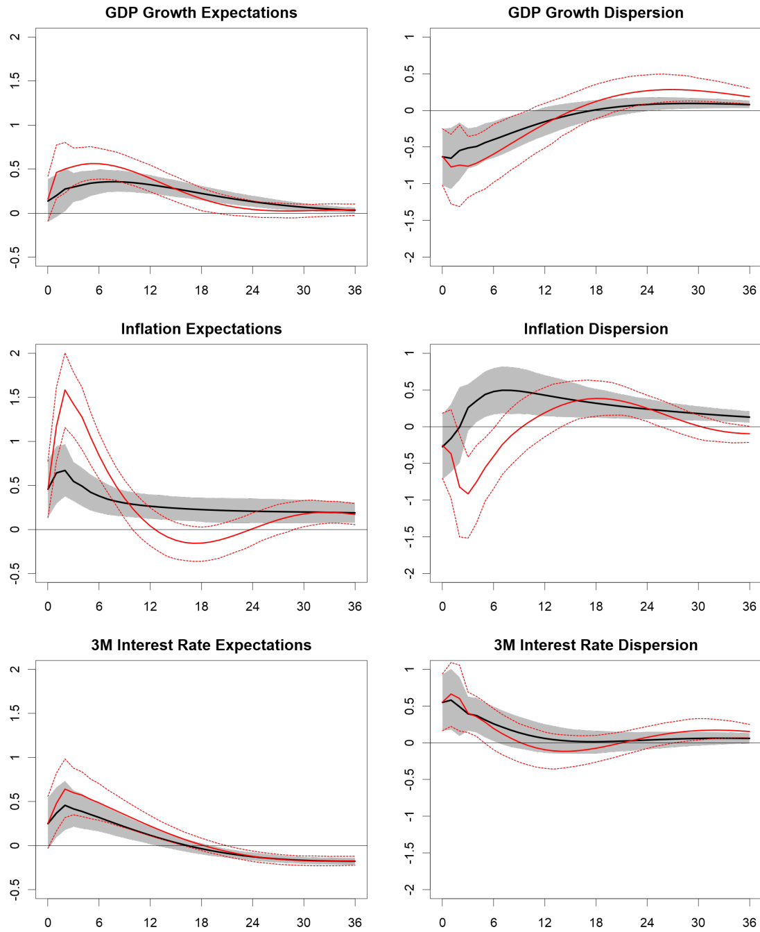
Figure 4: IRFs for Cyclical Value Factor ( \widetilde{HML} )
