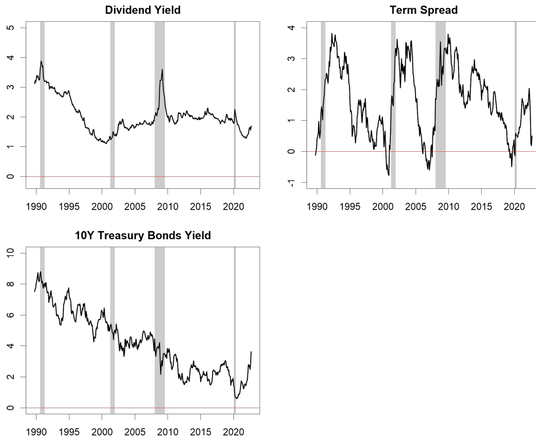
Figure A3: DAPM Predictors
