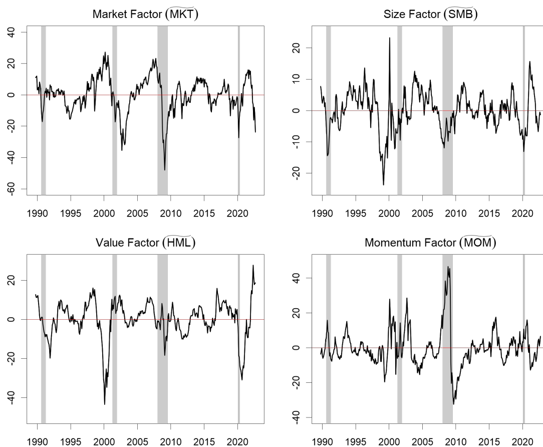
Figure A2: Cyclical Stock Market Factors
