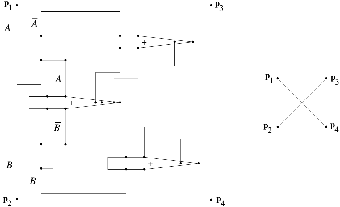
Figure 12: Crossing Two Transmission Lines
