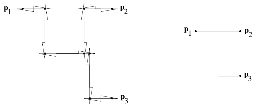
Figure 11: Splitter-Inverter
