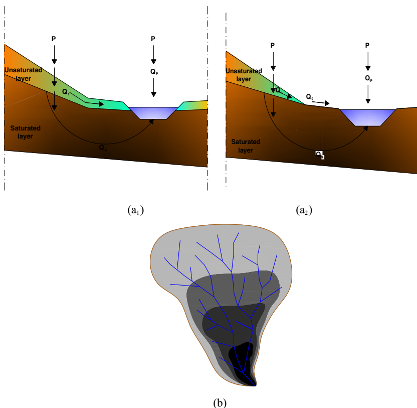
FIGURE 9.7 The runoff generation mechanism by saturation-excess. (A) Flow paths in the hillslope profile at the start ( a_1 ) and during ( a_2 ) precipitation ( P = precipitation; Q_p = direct precipitation over water surfaces; Q_o = overland flow; Q_t = interflow; Q_g = groundwater flow); (B) the progressive saturation mechanisms of the contributing areas (saturation degree increases with the gray intensity).
