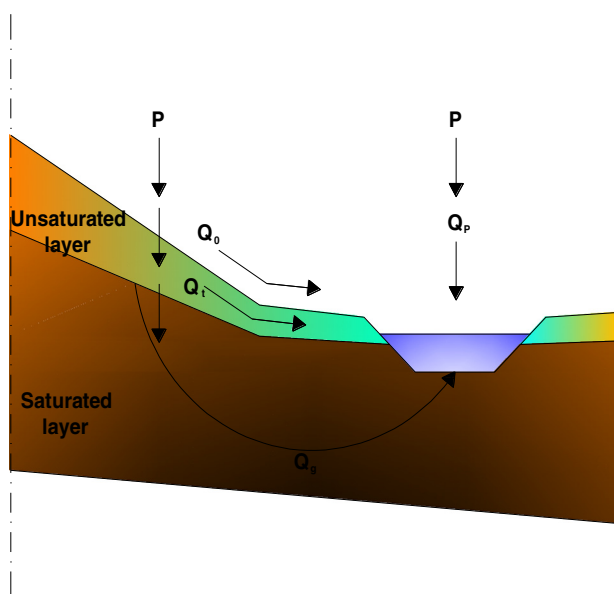
FIGURE 9.5 The different components of runoff along a hillslope ( P = precipitation; Q_p = direct precipitation over water surfaces; Q_o = overland flow; Q_i = interflow; Q_g = groundwater flow).
