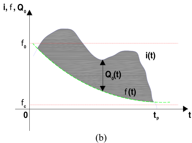
FIGURE 9.6 The runoff generation mechanism by infiltration excess. (A) Flow paths in the hillslope profile ( P = precipitation; Q_p = direct precipitation over water surfaces; Q_o = overland flow); (B) the theoretical diagram ( f = infiltration rate; f_c = steady infiltration rate; f_0 = initial infiltration rate; t_p = precipitation duration; i = precipitation intensity; Q_o = overland flow).
