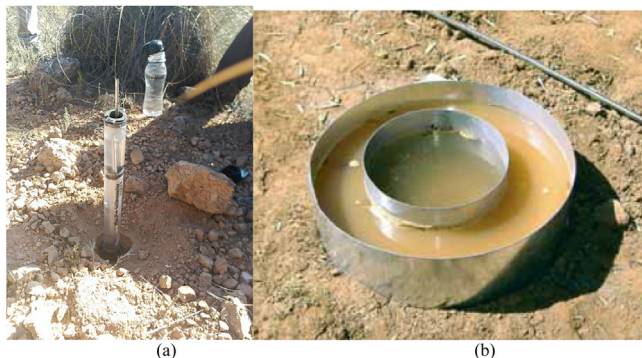
FIGURE 9.13 Minidisk infiltrimeter (Decagon Inc., USA, A) and double-ring infiltrimeter (B).
